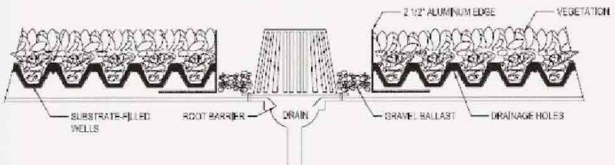
Roof Drain Detail
