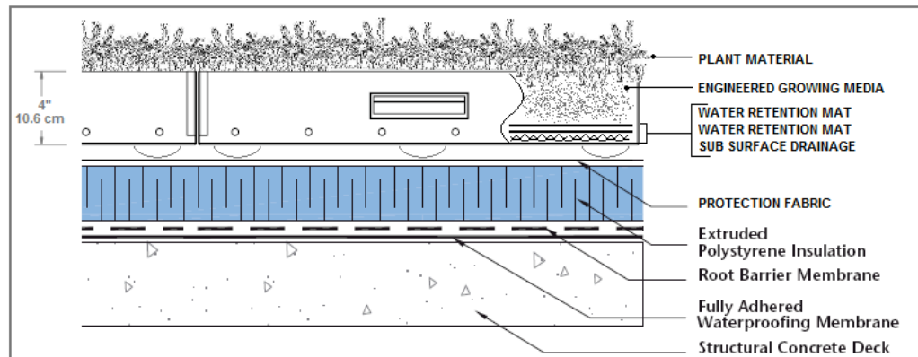
GREEN LIVING™ ROOF TRAY PROTECTED MEMBRANE APPLICATION
